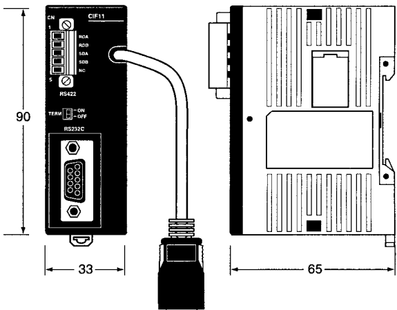
RS-422/RS-232C Adapter Unit (CPM2C-CIF11)
